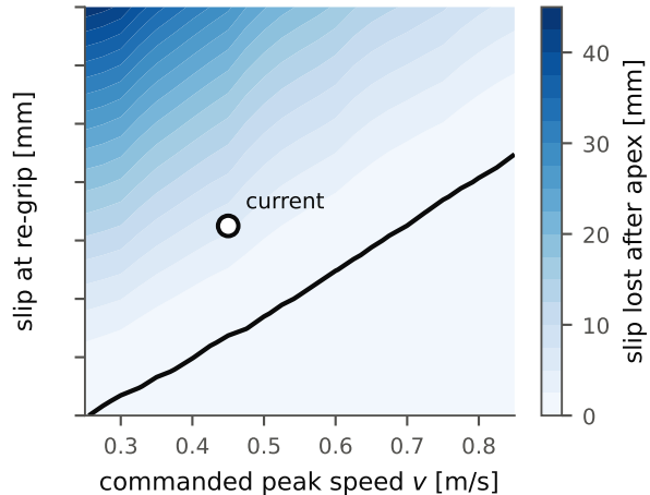
(b) cost of a pulse that outlasts the apex
