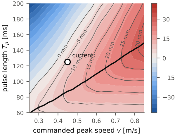
(a) slip, black line: w = 0 at re-grip
