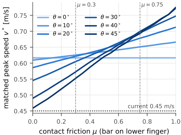
(a) v^* for T_p = 125 ms, full chain
