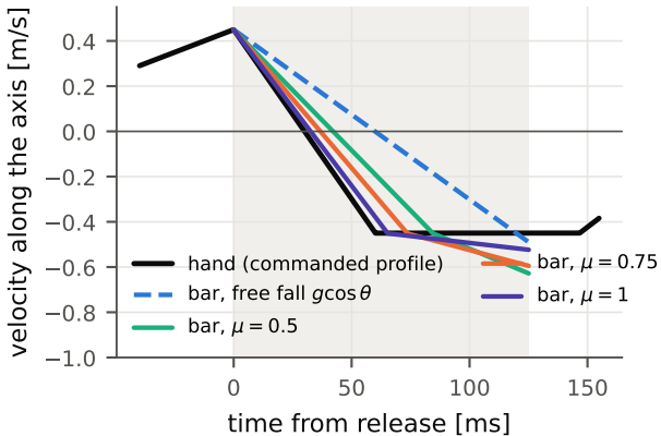
(a) velocities during the pulse
