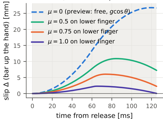
(b) slip, \theta = 40^\circ , T_p = 125 ms
