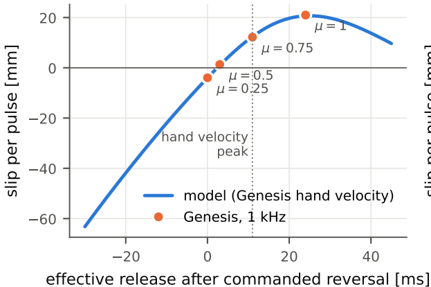
(a) \theta = 0^\circ : slip is set by release timing
