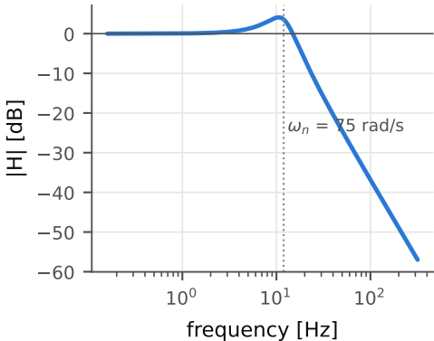
(a) H(s) = \omega_n^2 / (s^2 + 2\zeta\omega_n s + \omega_n^2)
