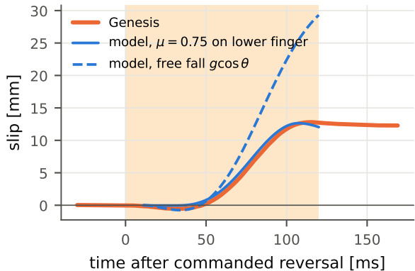
(b) slip: Genesis vs 1-D model
