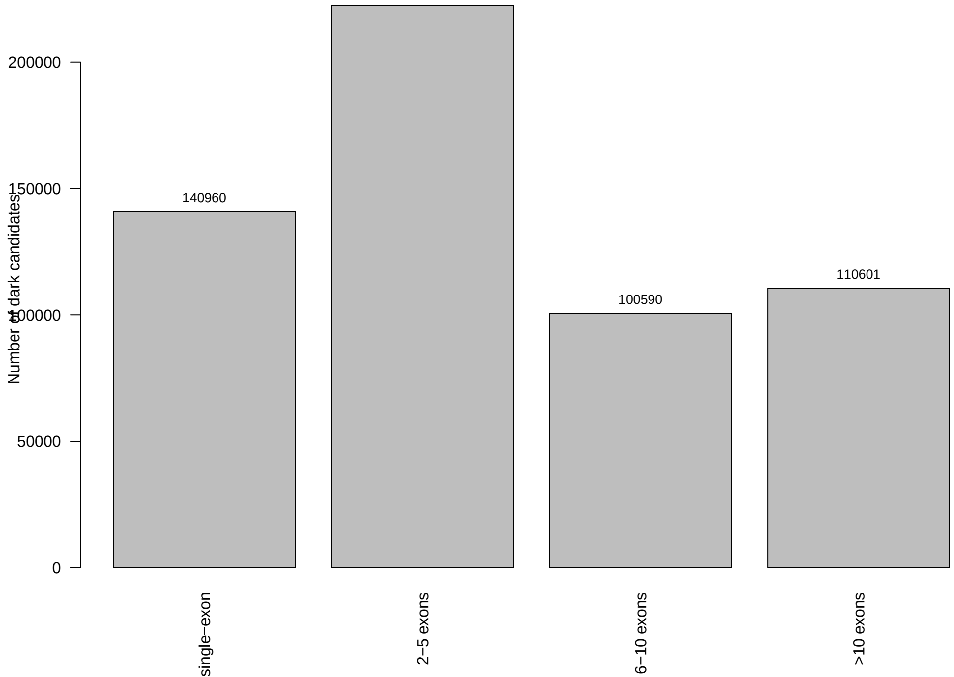
Exon count distribution of genome-linked dark candidates
