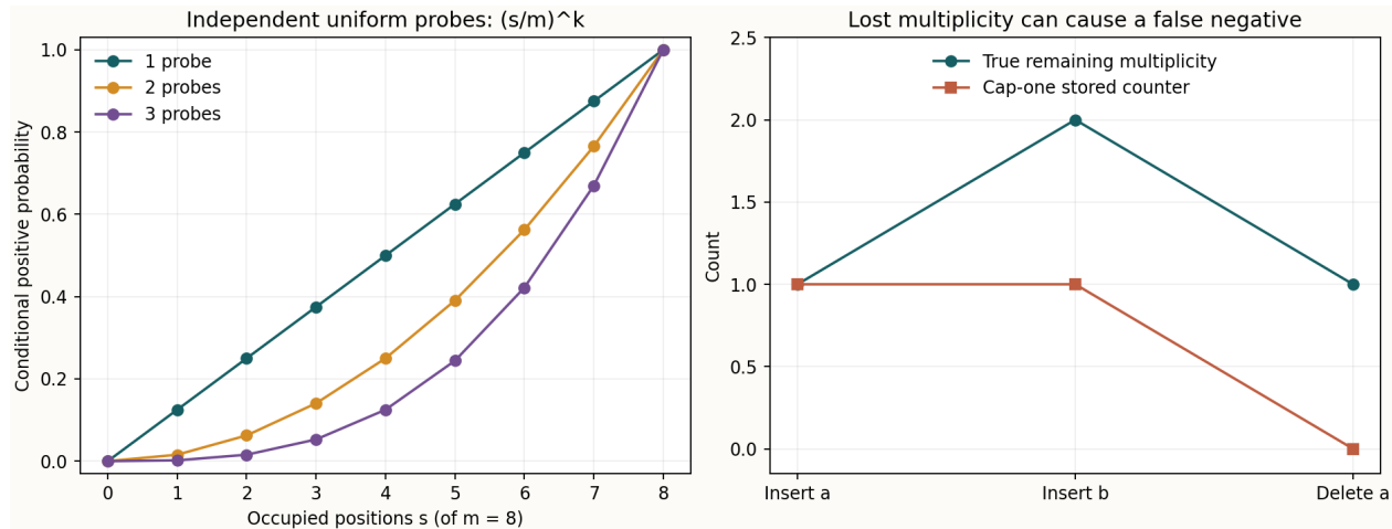
Deterministic arithmetic and a retained finite counterexample; no empirical data.
