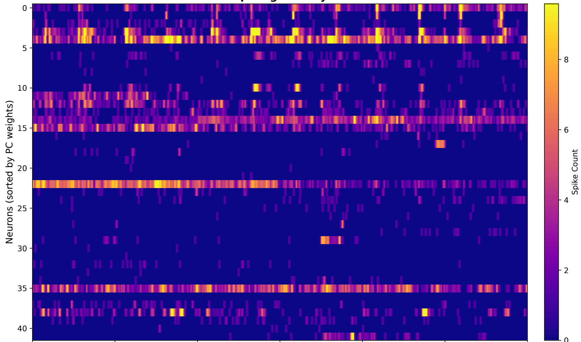
Spiking Activity
