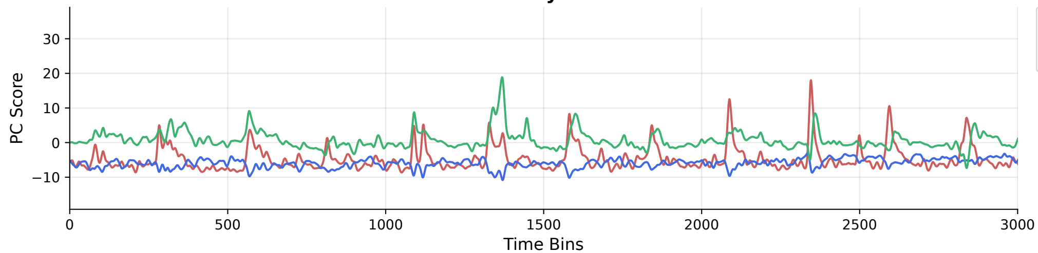
Latent Dynamics
