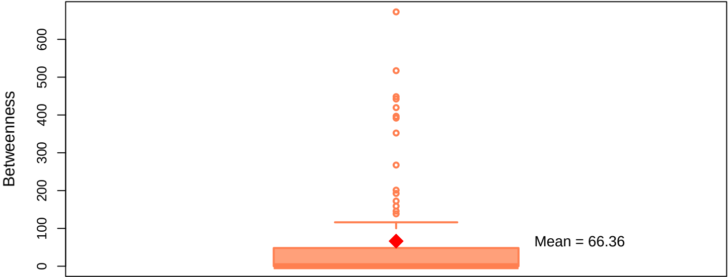
Betweenness Centrality – Boxplot
