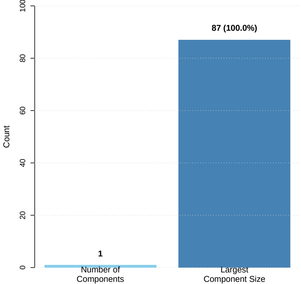
Network Components
