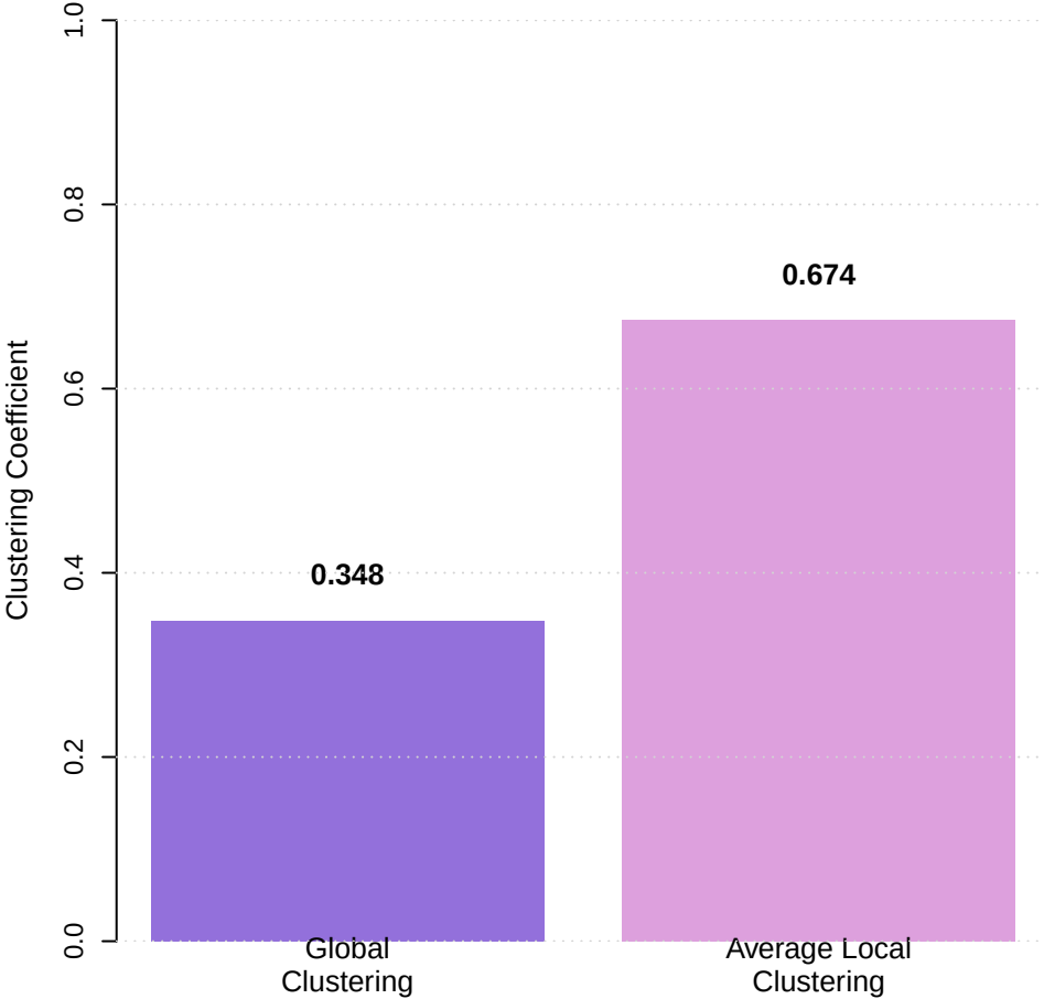
Clustering Coefficients
