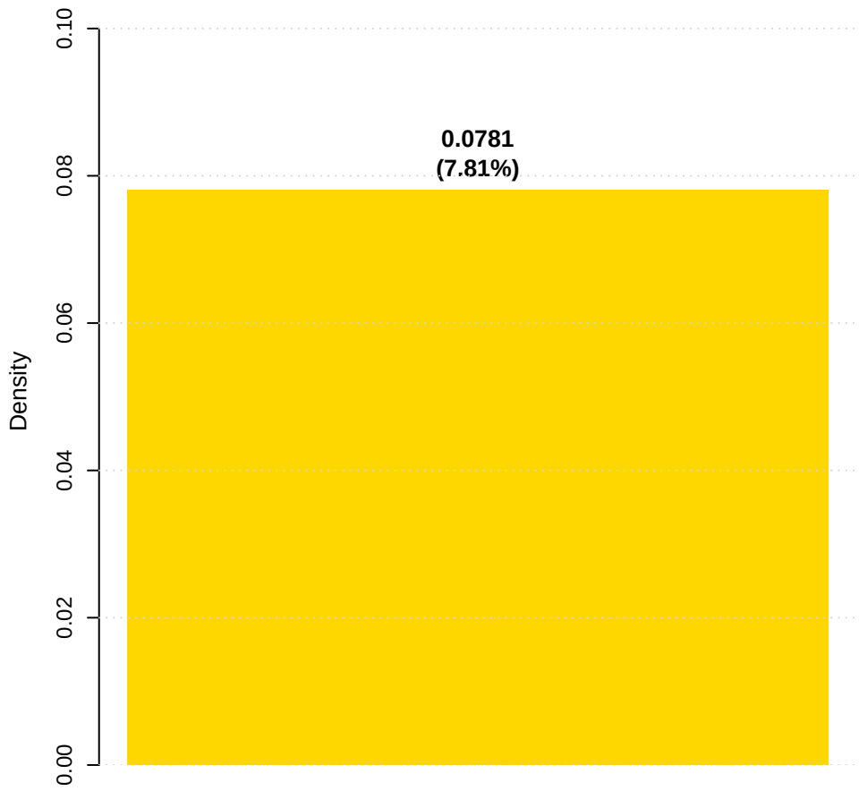
Network Density
