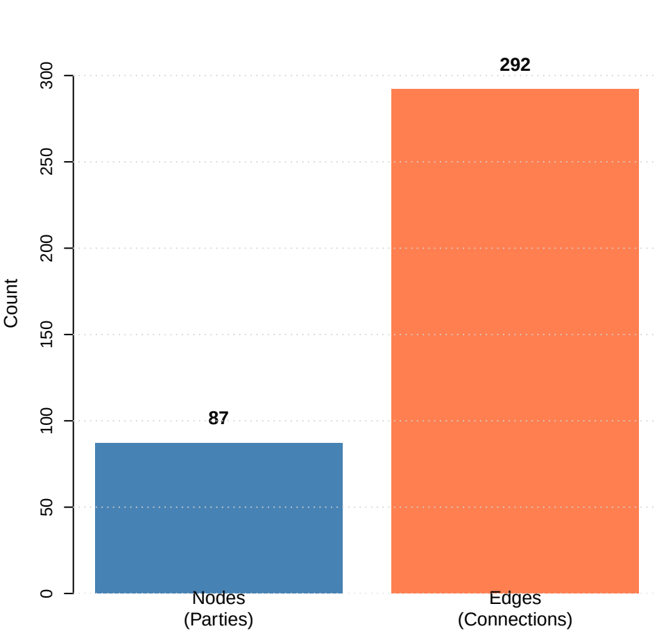
Network Size
