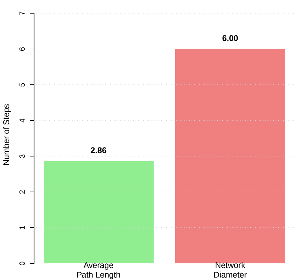
Path Metrics
