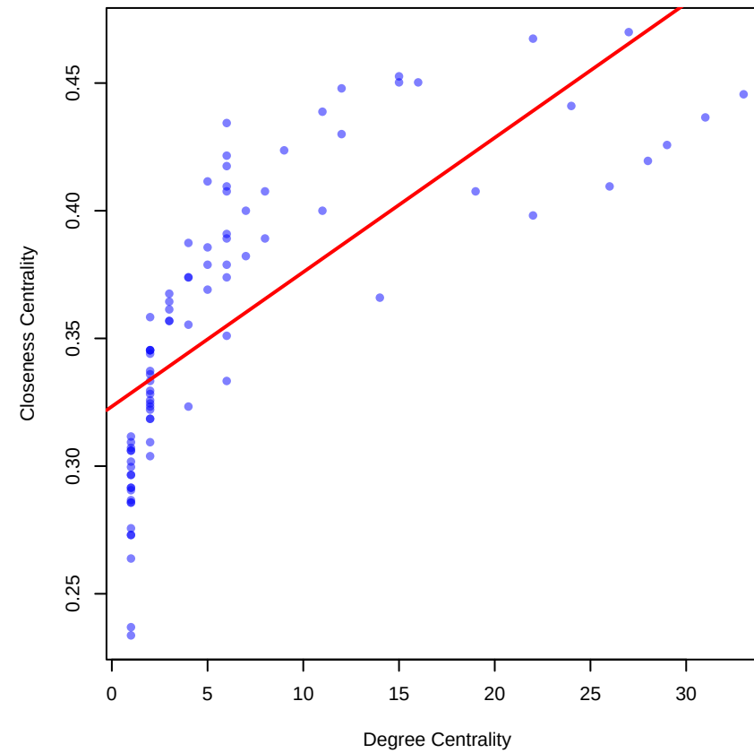
Degree vs Closeness
