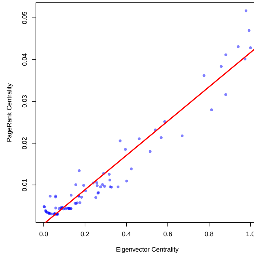
Eigenvector vs PageRank
