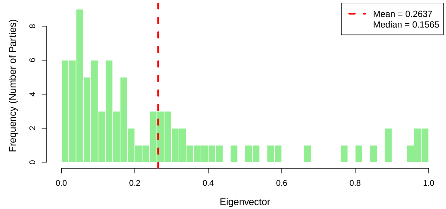
Eigenvector Distribution
