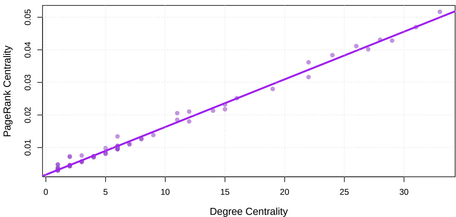
PageRank vs Degree
