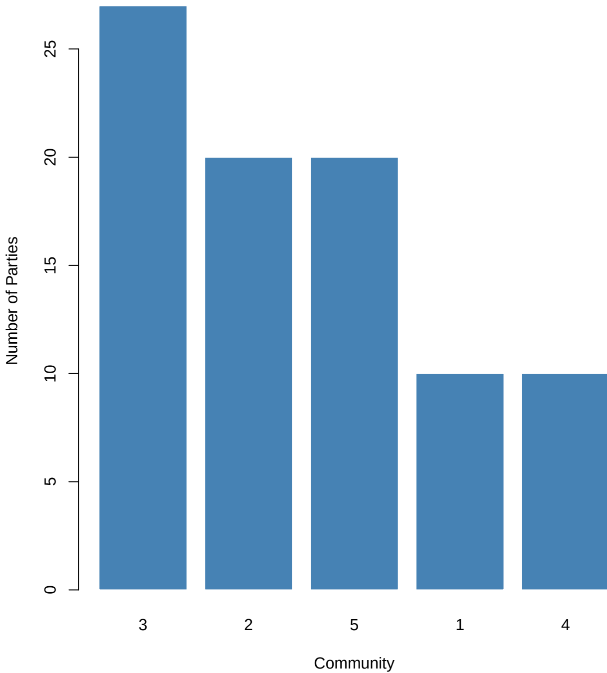
Louvain Community Sizes 5 communities, Modularity = 0.241
