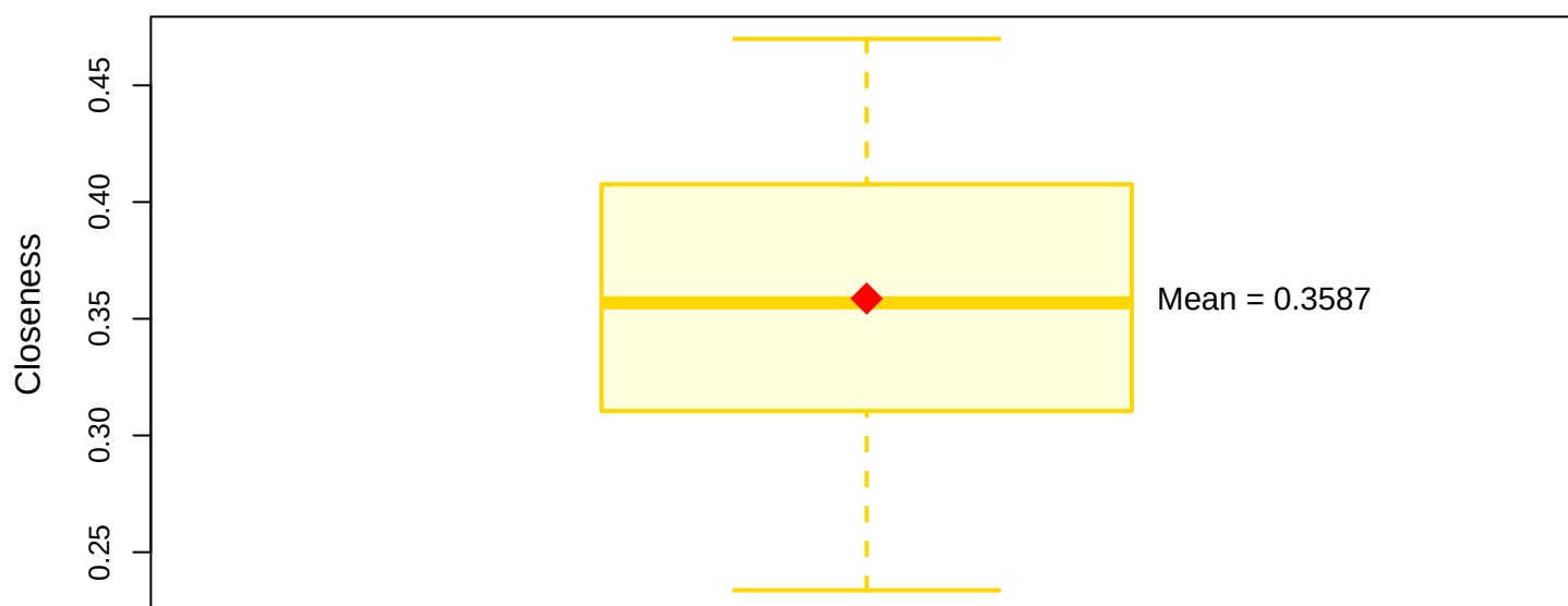
Closeness Centrality – Boxplot
