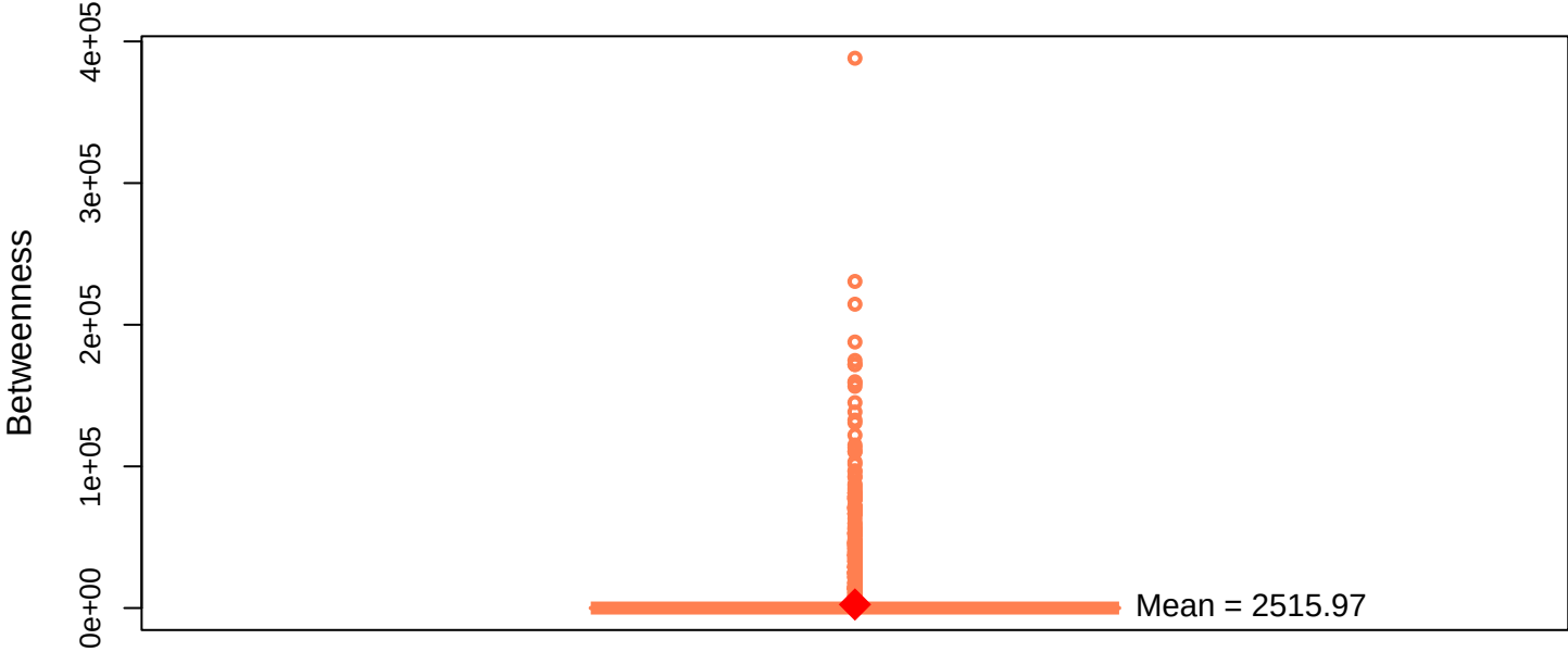
Betweenness Centrality – Boxplot
