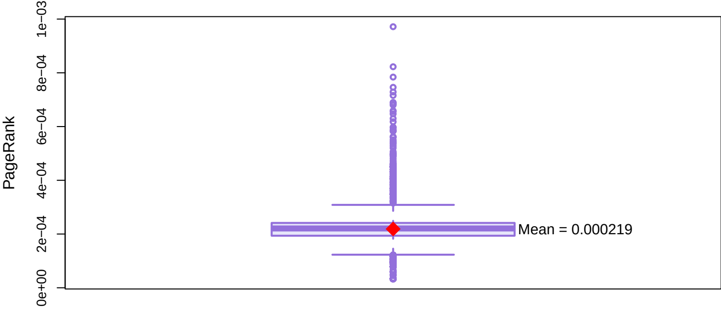
PageRank Centrality – Boxplot
