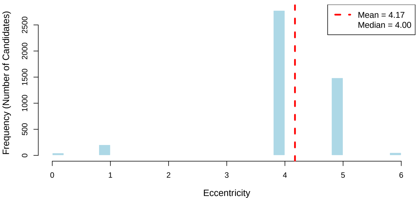
Eccentricity Distribution
