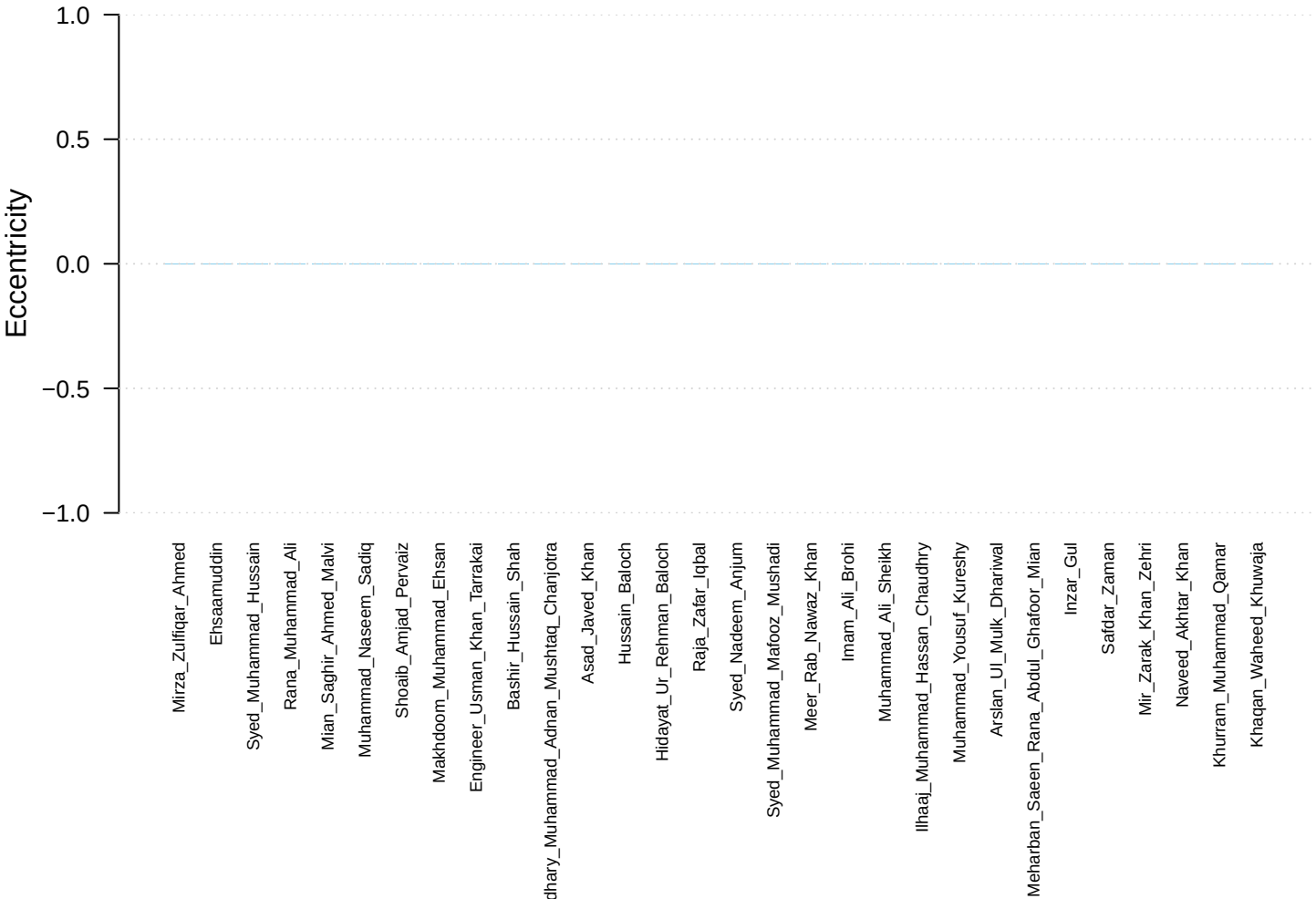
Eccentricity – Boxplot
