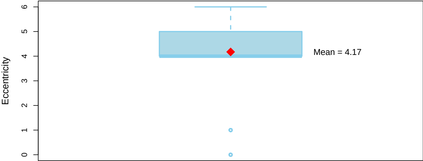
Eccentricity – Boxplot
