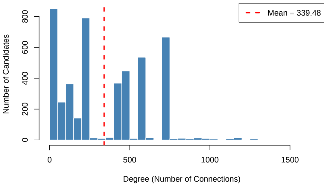
Degree Distribution – Candidate–Candidate Network
