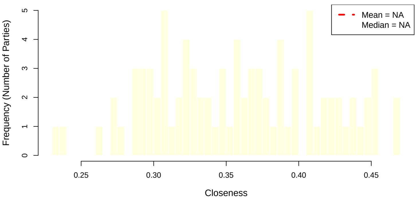
Closeness Distribution
