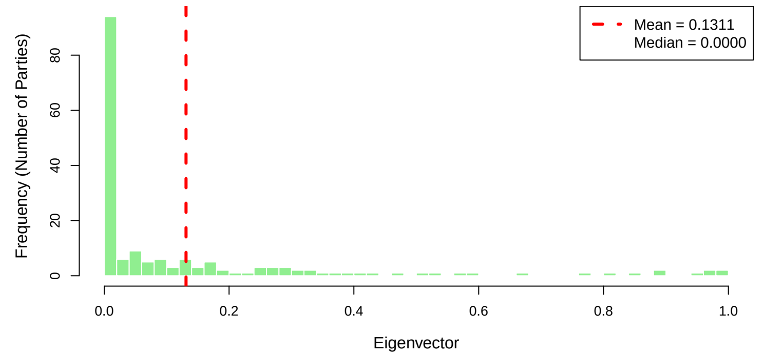
Eigenvector Distribution
