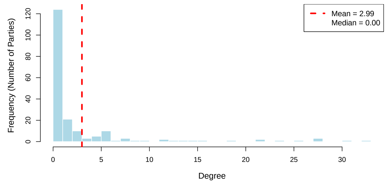
Degree Distribution
