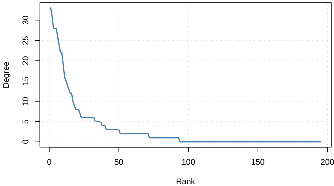
Cumulative Degree Distribution
