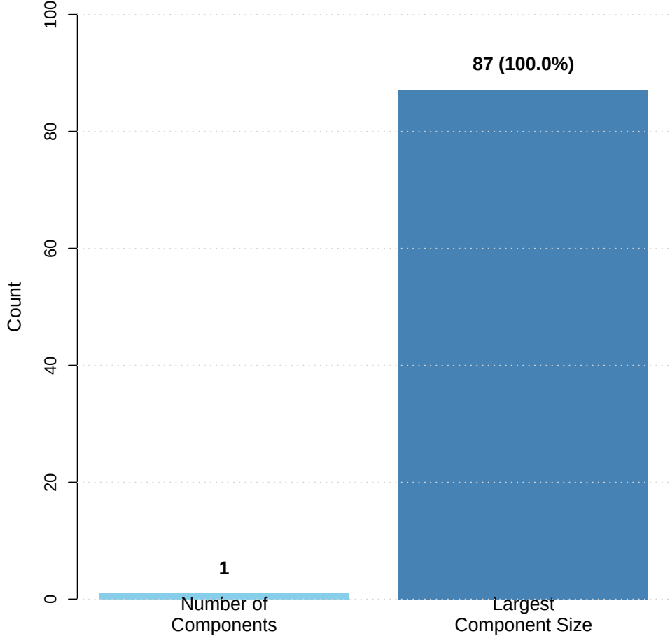
Network Components
