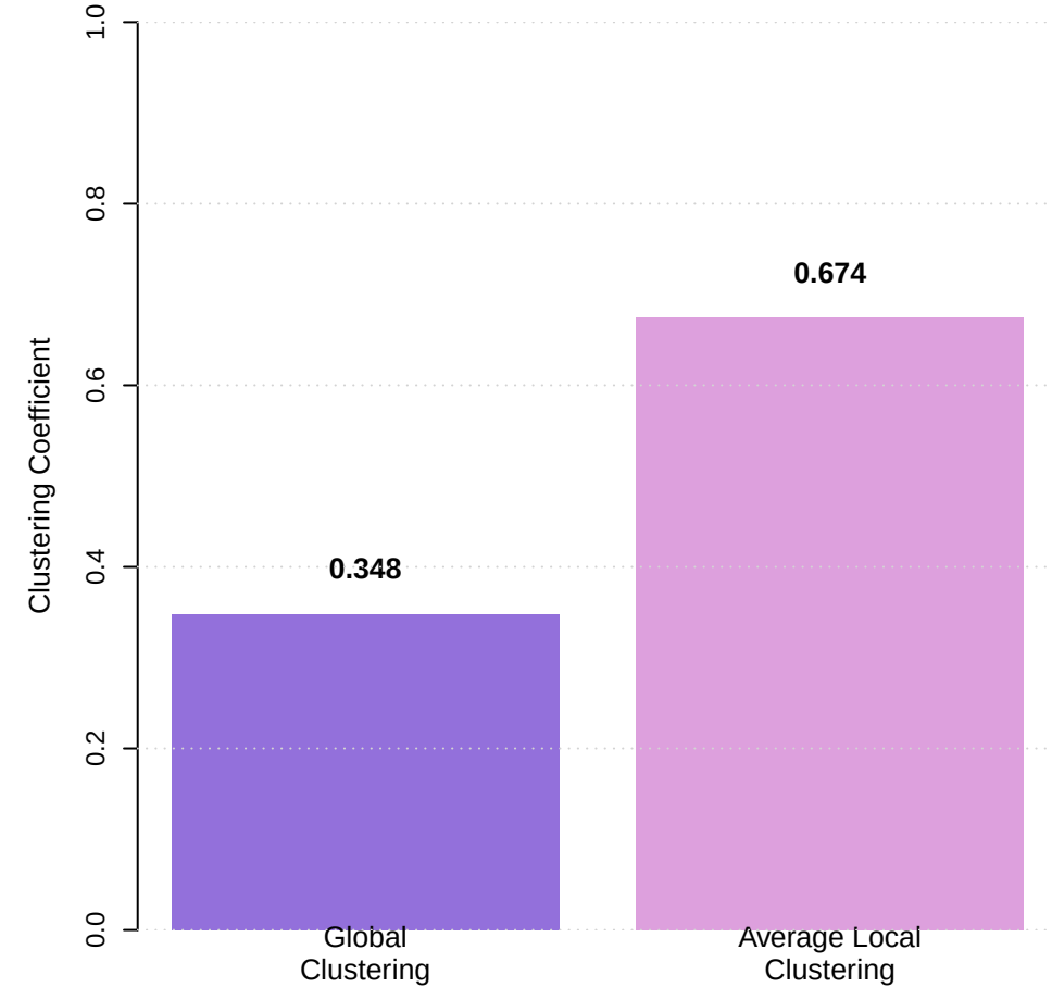
Clustering Coefficients
