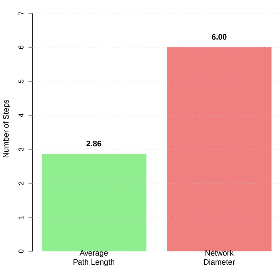
Path Metrics
