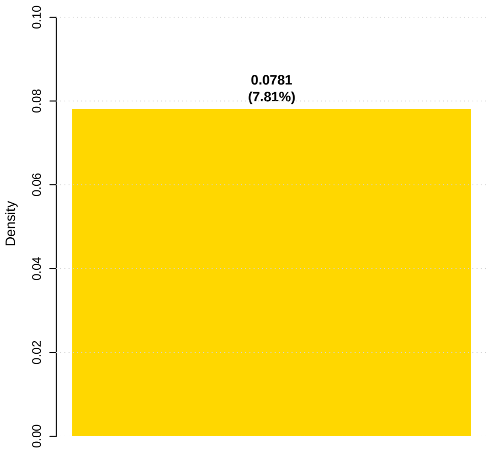
Network Density
