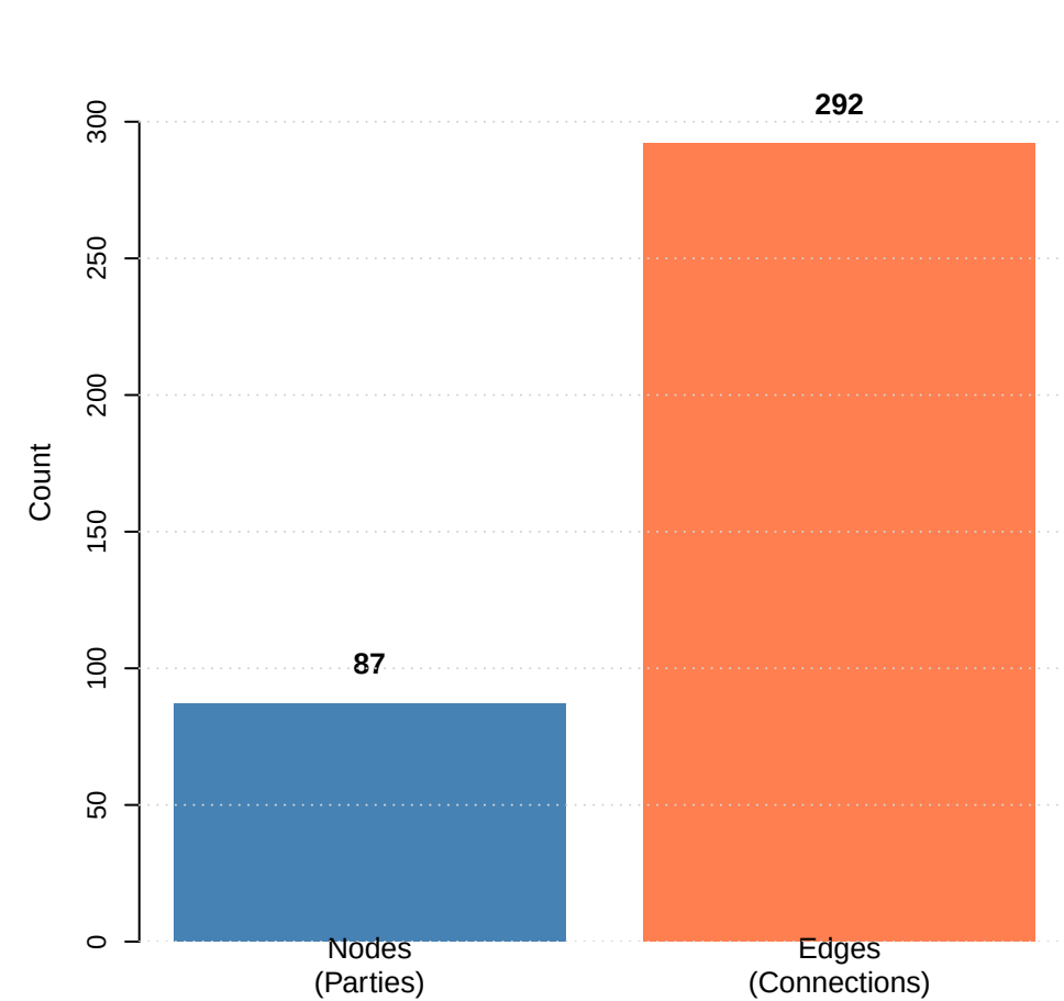
Network Size
