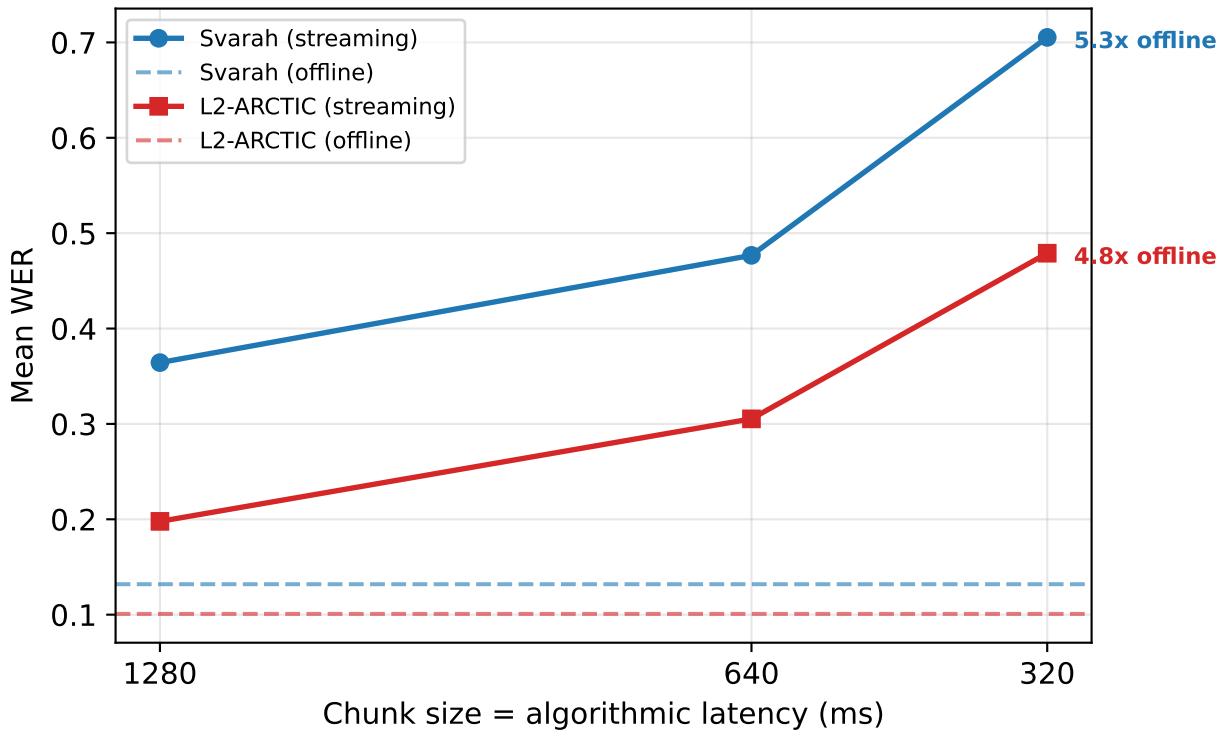
Streaming latency vs WER
