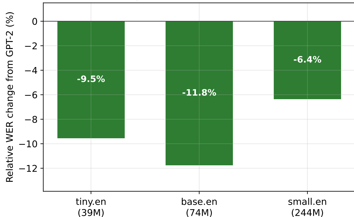
GPT-2 gain holds across ASR model size
