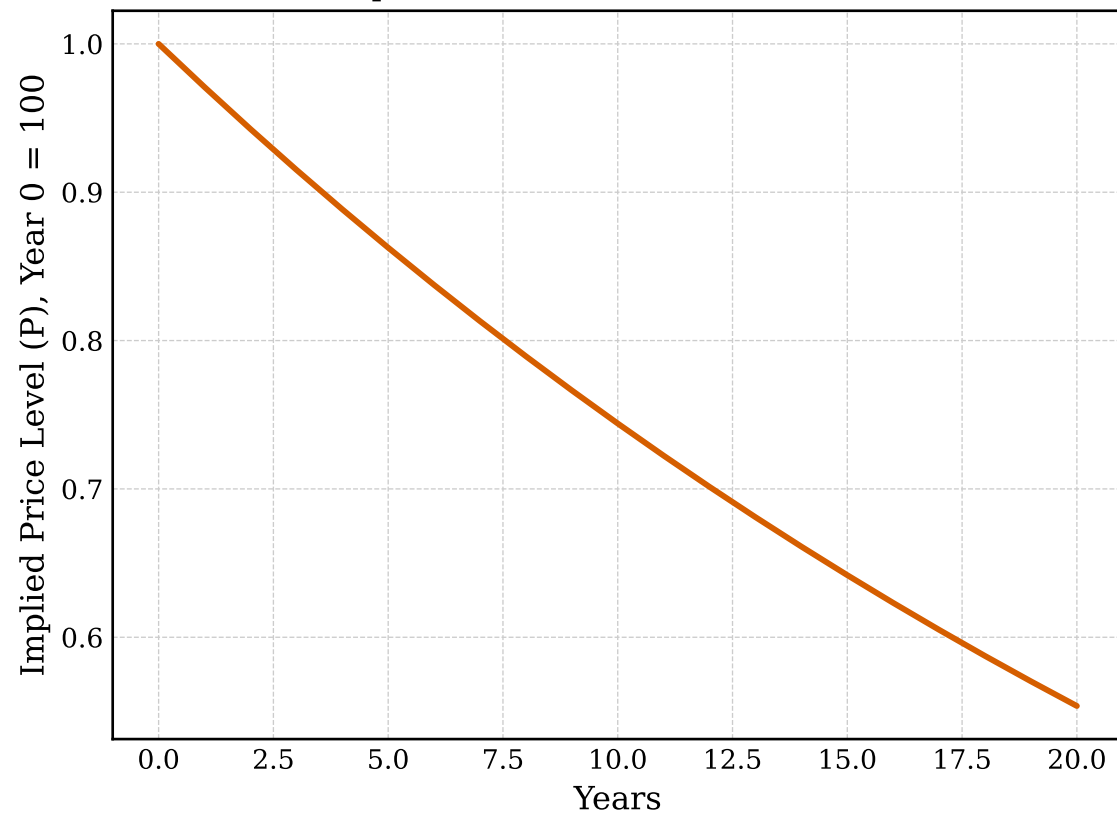
Implied Price Level from M \cdot V = P \cdot Y
