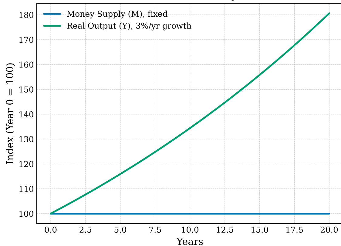
Fixed M vs. Growing Y
