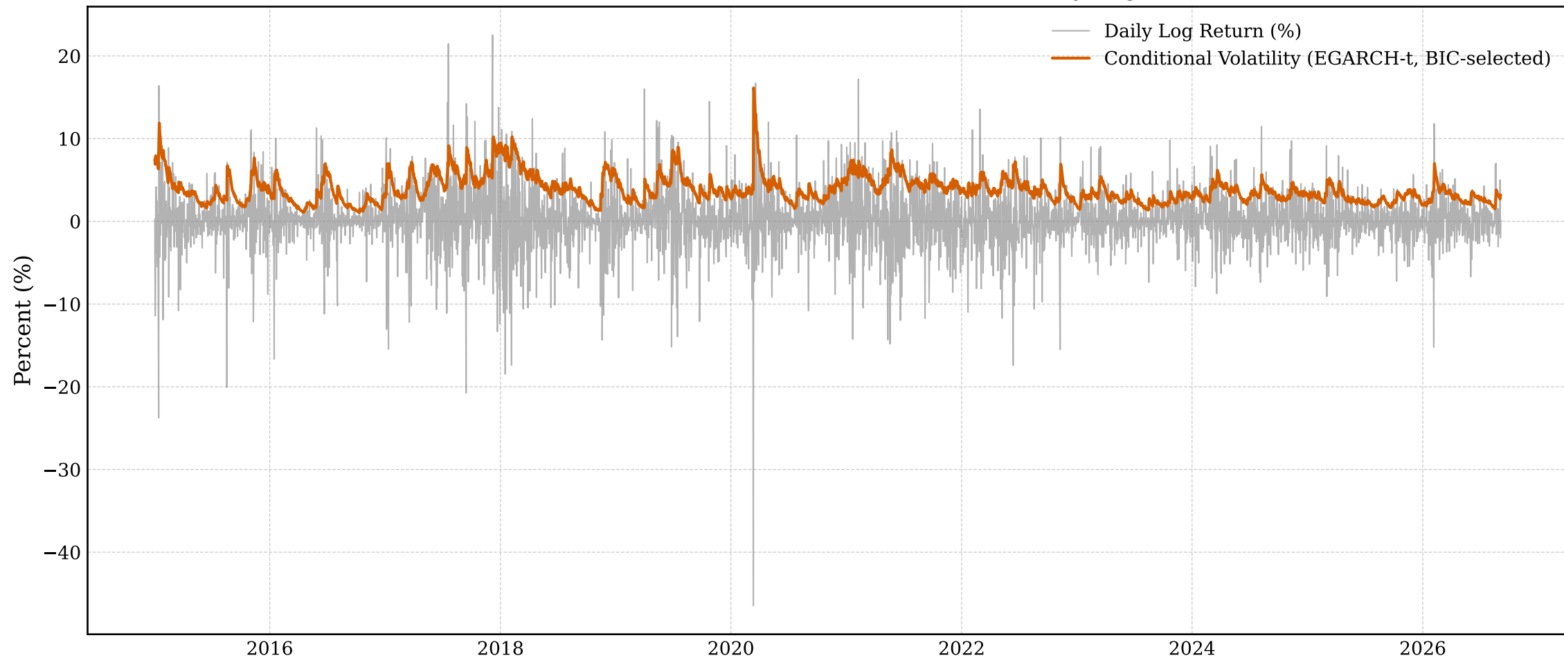
Bitcoin Returns and BIC-Selected Conditional Volatility (Fig. A3)
