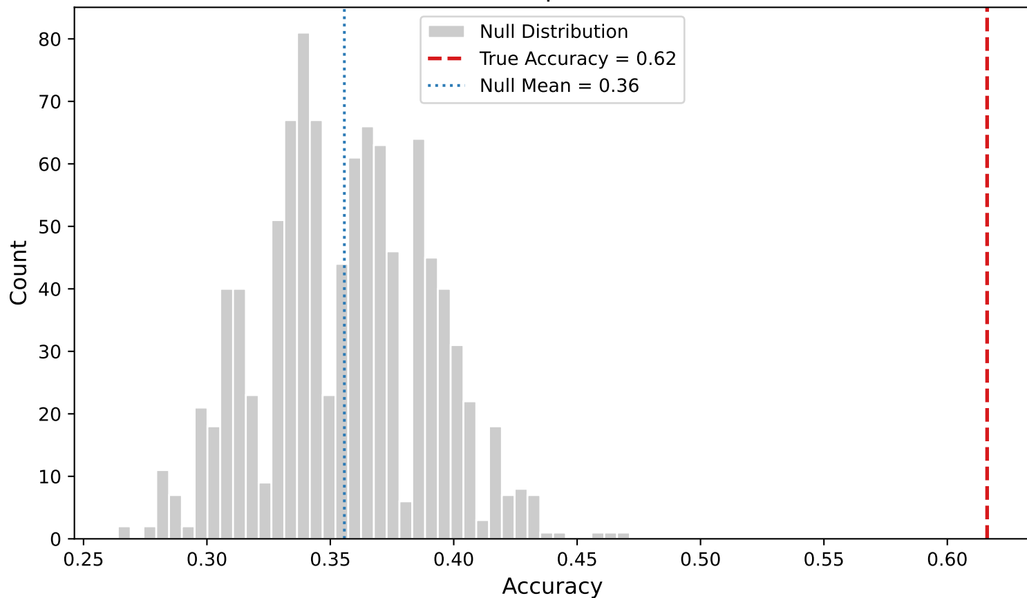
RF Permutation Test ( p = 0.0010 , n = 1000 )
