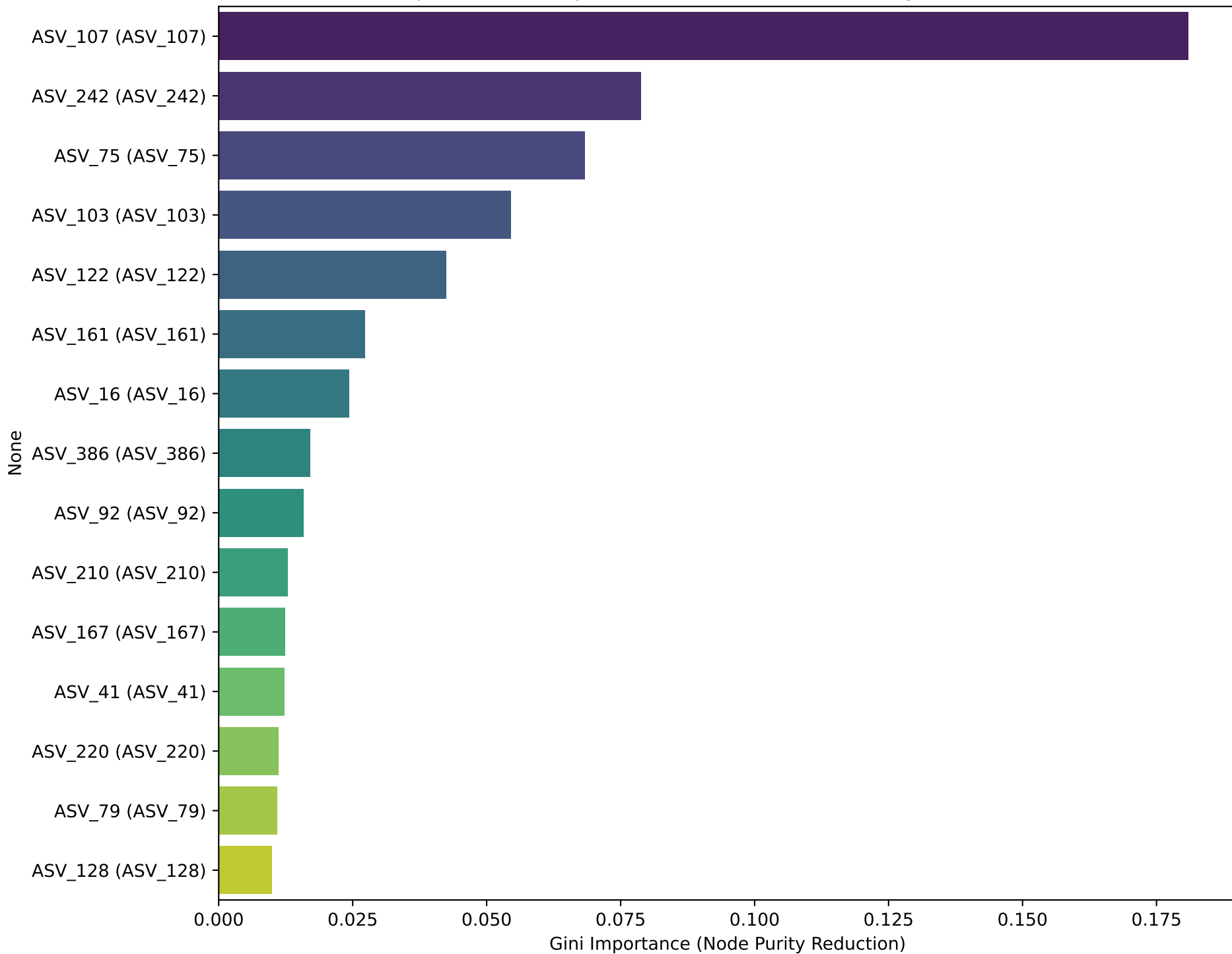
Top 15 Strict-Temporal Taxonomic Biomarkers (Age-of-Isolation)
