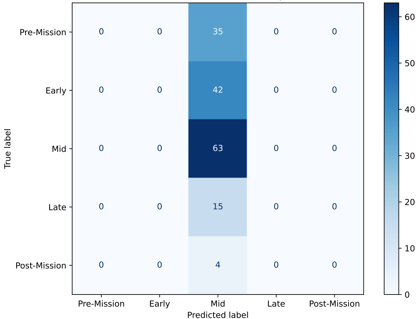
LP-Micro LOSO Confusion Matrix XGBoost on Group-Lasso Features | Acc = 0.396
