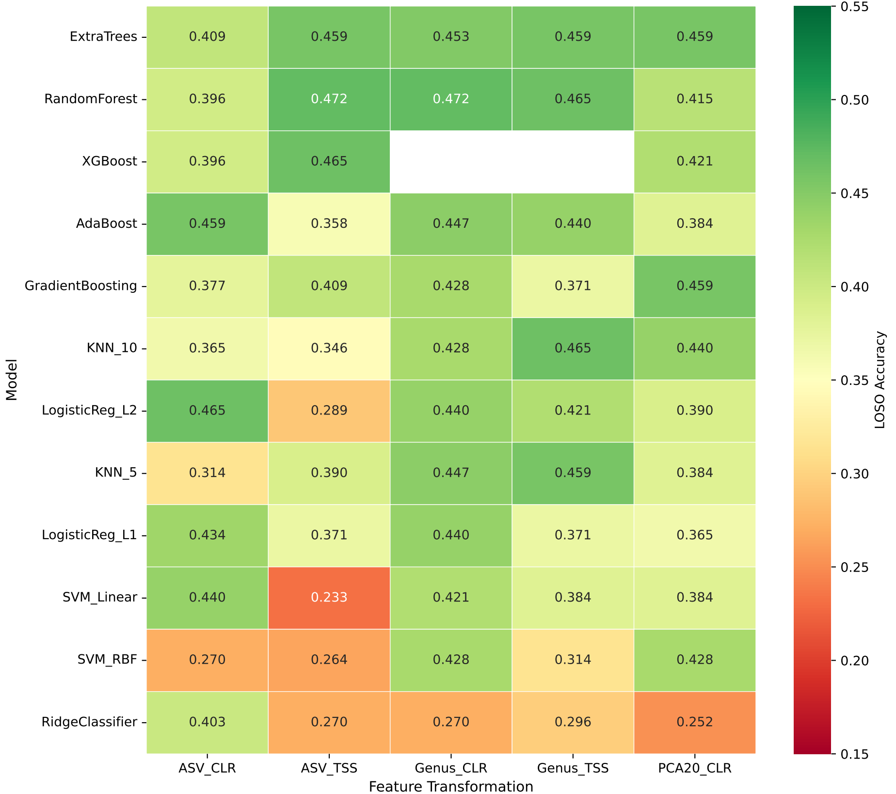
Phase Classification — Multi-Model × Multi-Feature LOSO Benchmark
