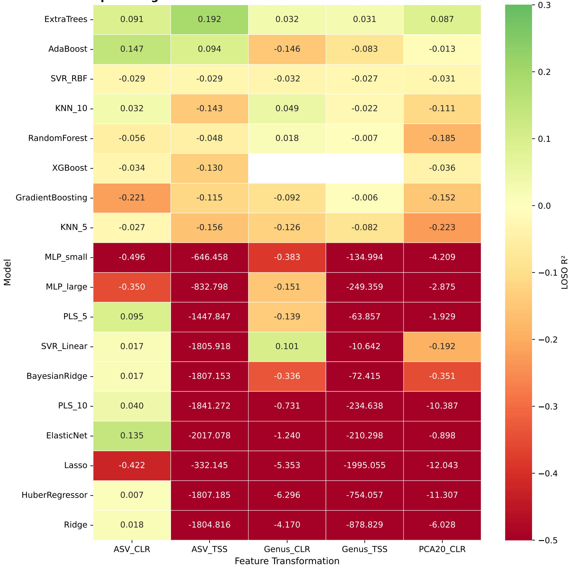
Temporal Regression — Multi-Model × Multi-Feature LOSO Benchmark
