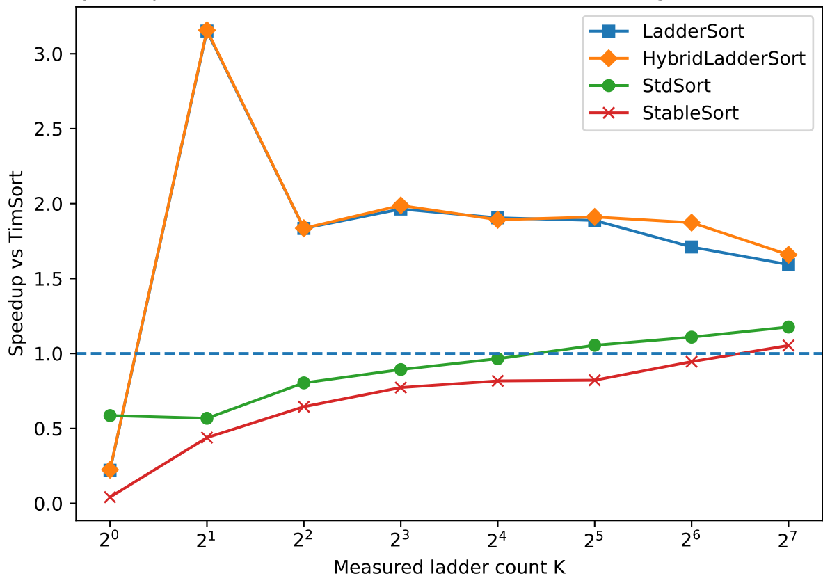
Speedup vs TimSort, randomized exact-K interleaving, N=10000000
