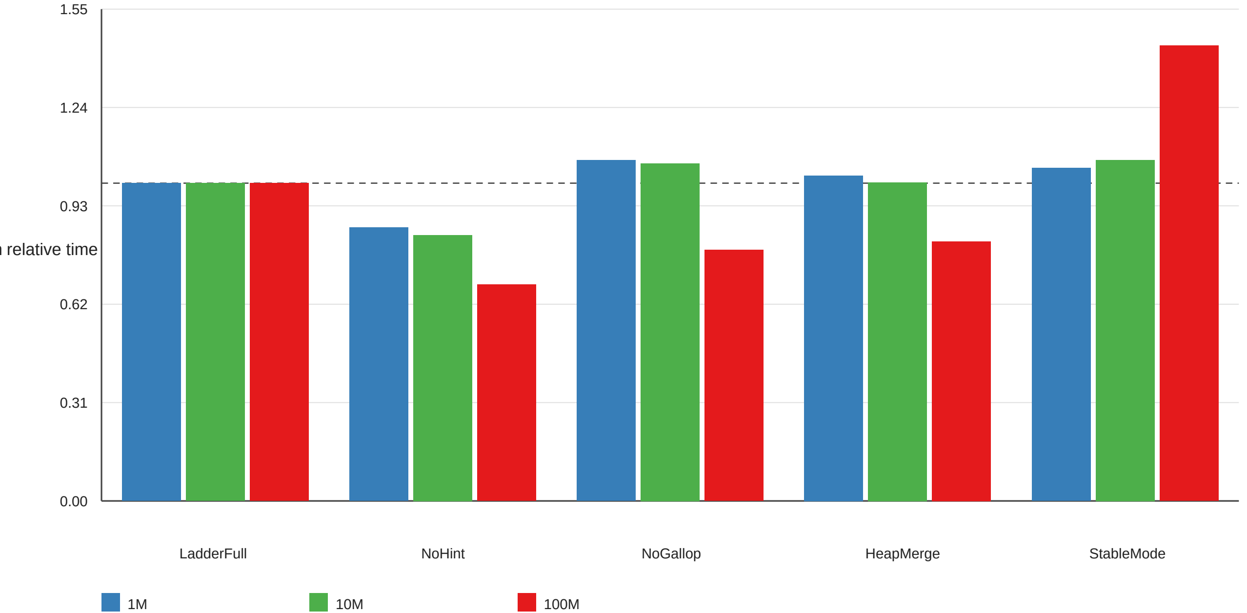
Two-Run Riffle Ablation: Median Relative Time
