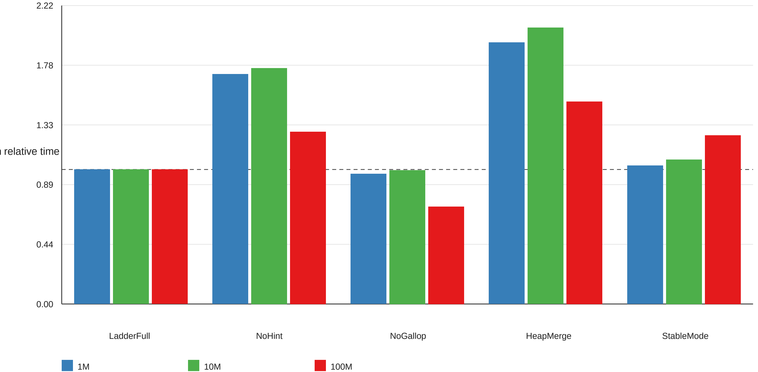
Social Feed Ablation: Median Relative Time
