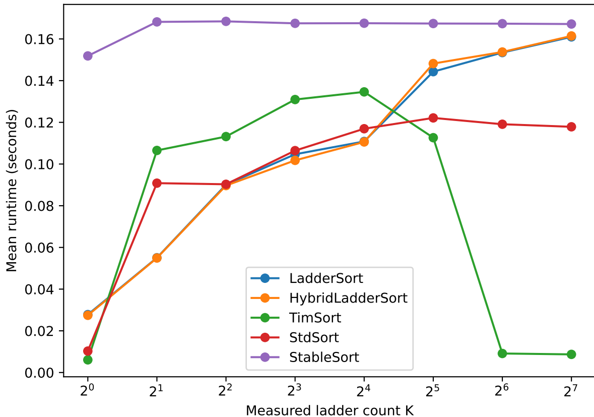
Runtime vs measured K, N=10000000
