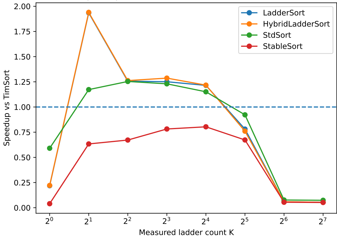
Speedup vs TimSort as K varies, N=10000000
