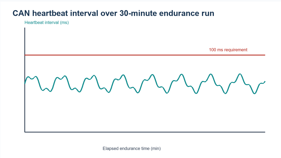
Figure 4. Heartbeat interval remained below 100 ms for the full 30-minute run; message counter showed zero loss.
