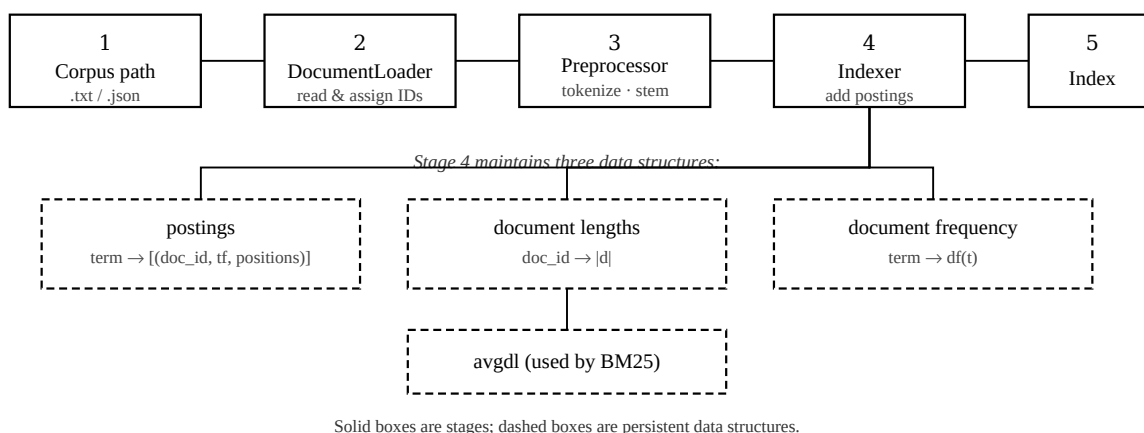
Figure 2. Stages and persistent data structures of the indexing pipeline.
