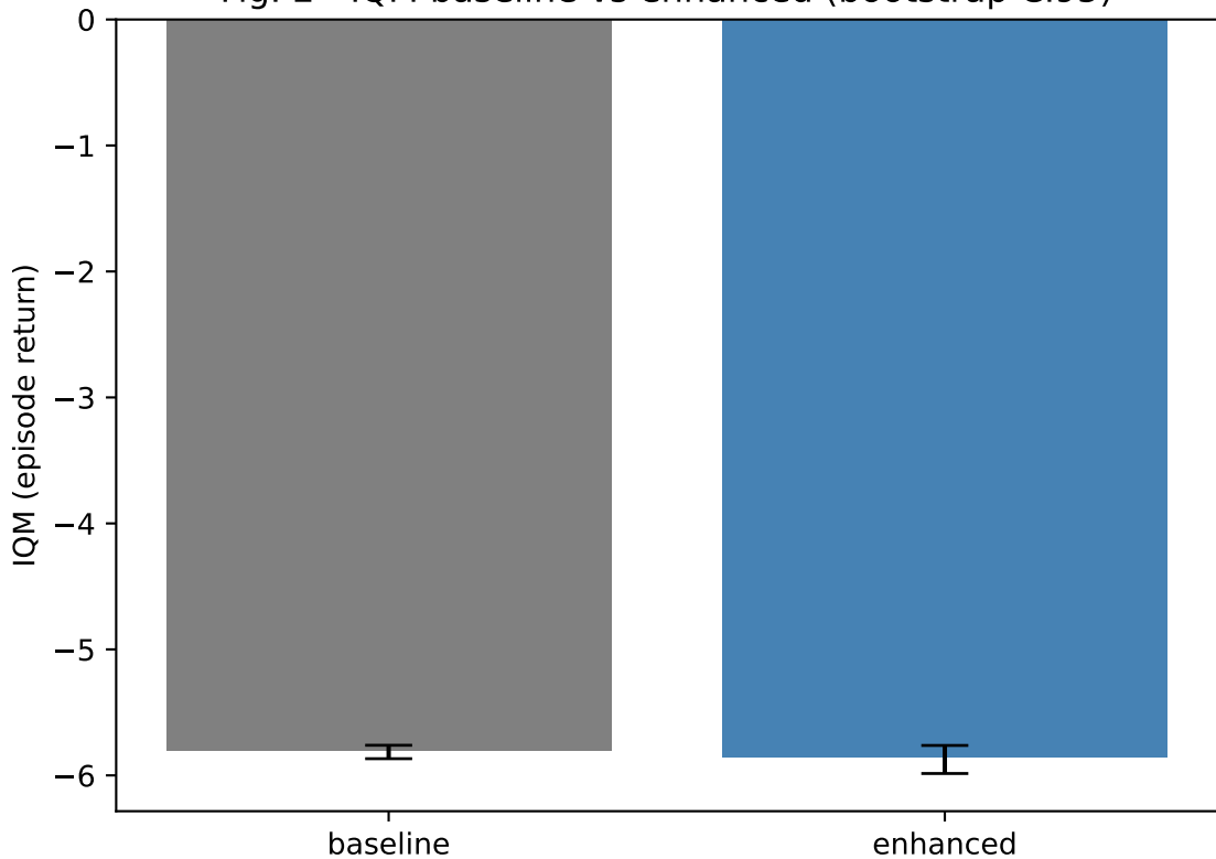
Fig. 2 - IQM baseline vs enhanced (bootstrap CI95)
