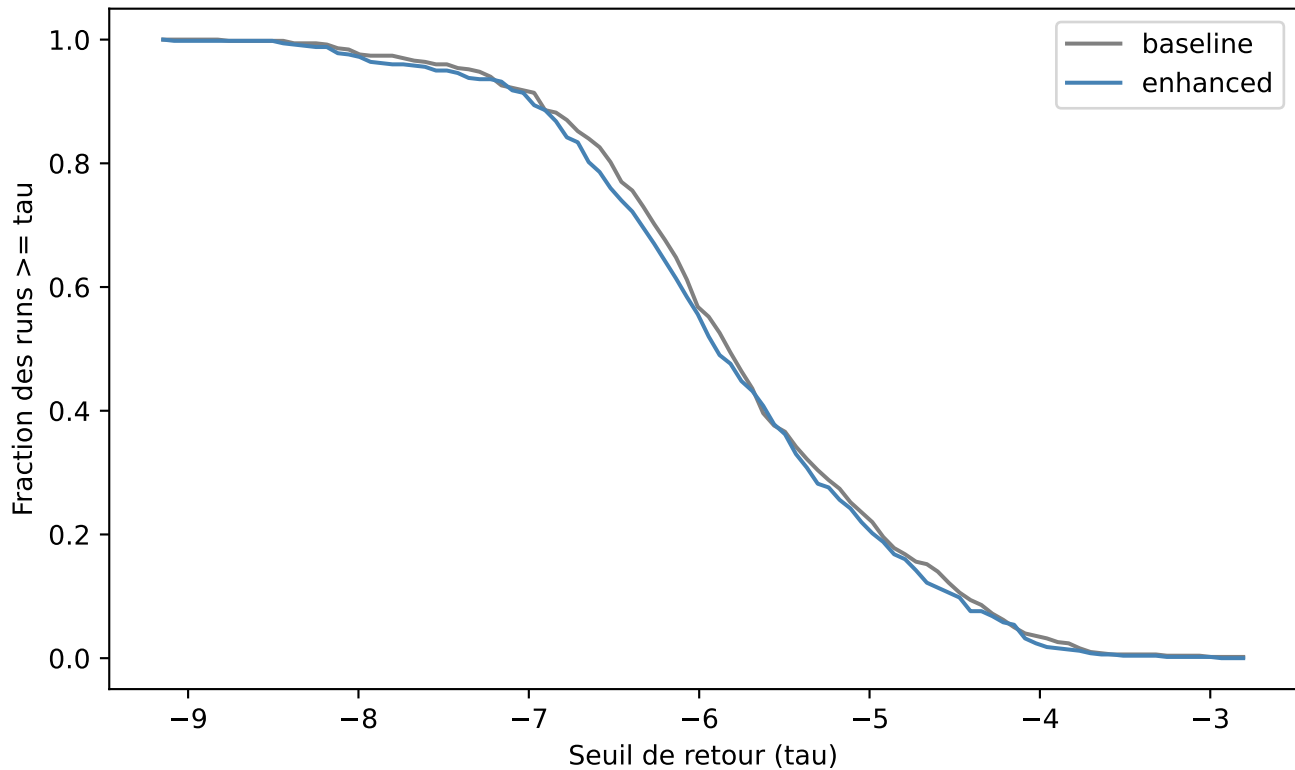
Fig. 3 - Performance profile
