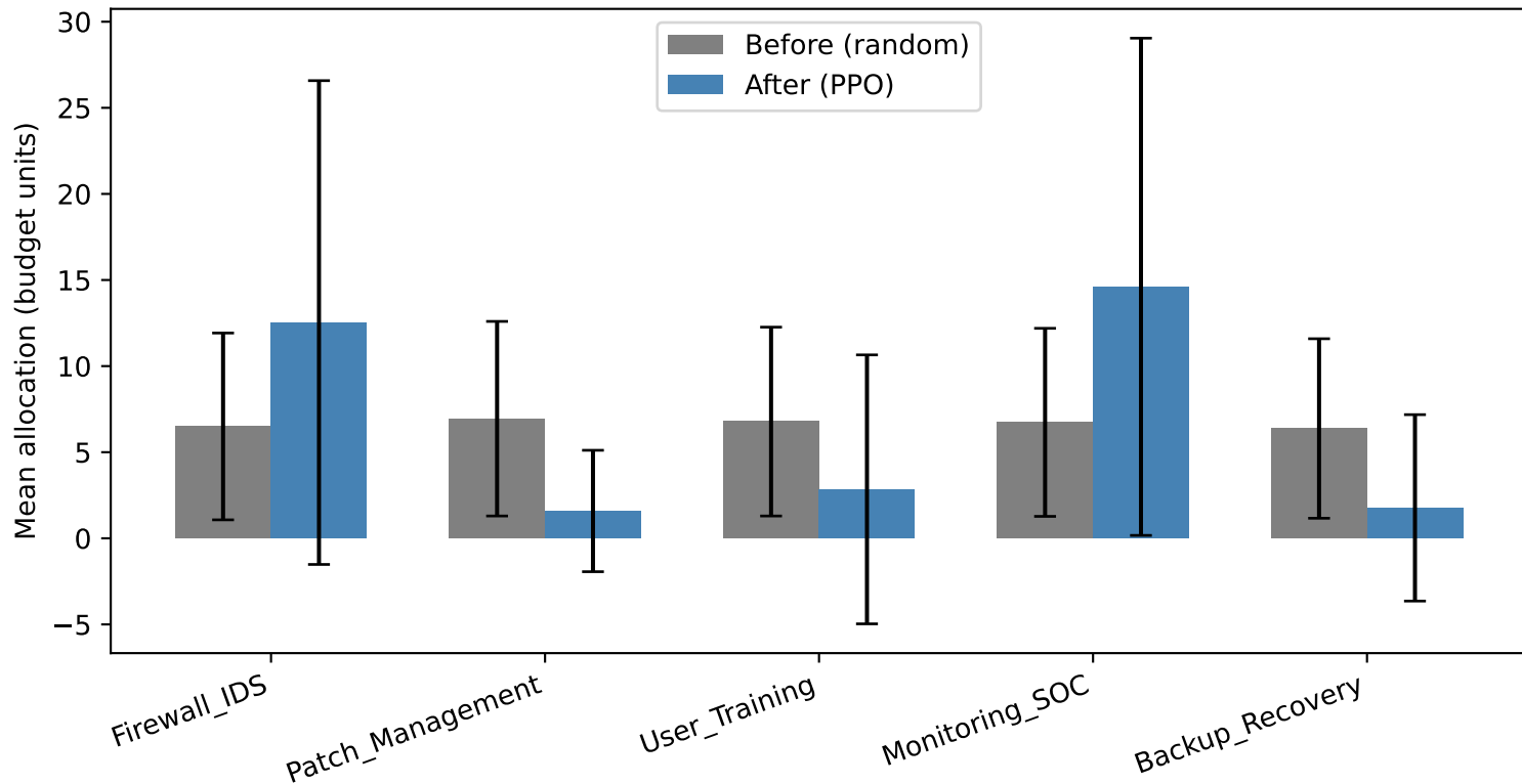
Fig. 5 - Mean allocation per resource, before vs after training (n=30 episodes)
