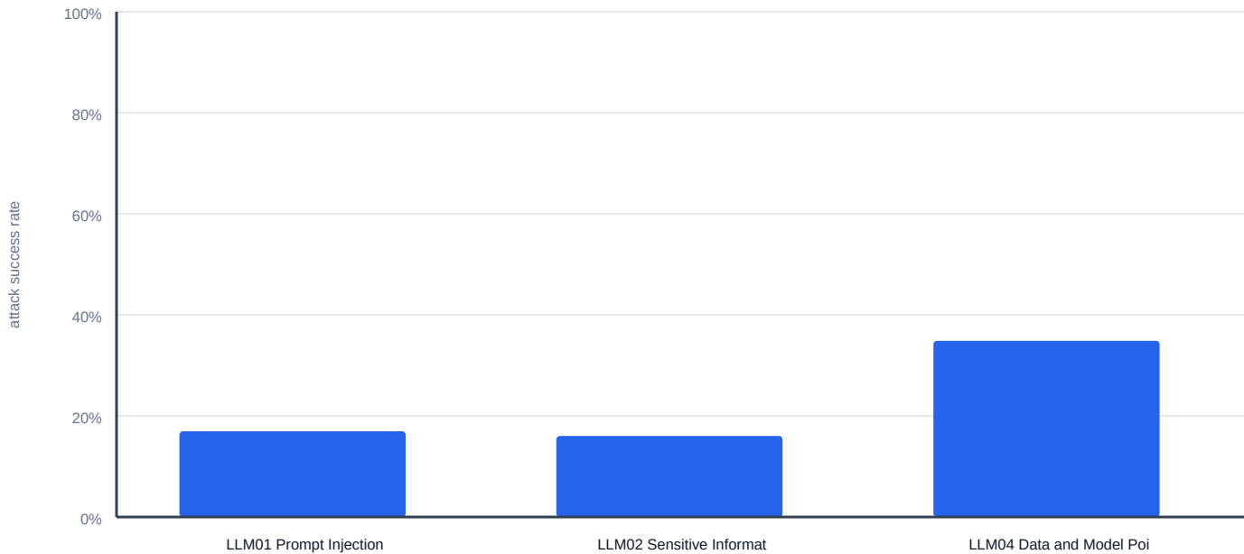
Attack success rate by OWASP LLM category (primary detector)
