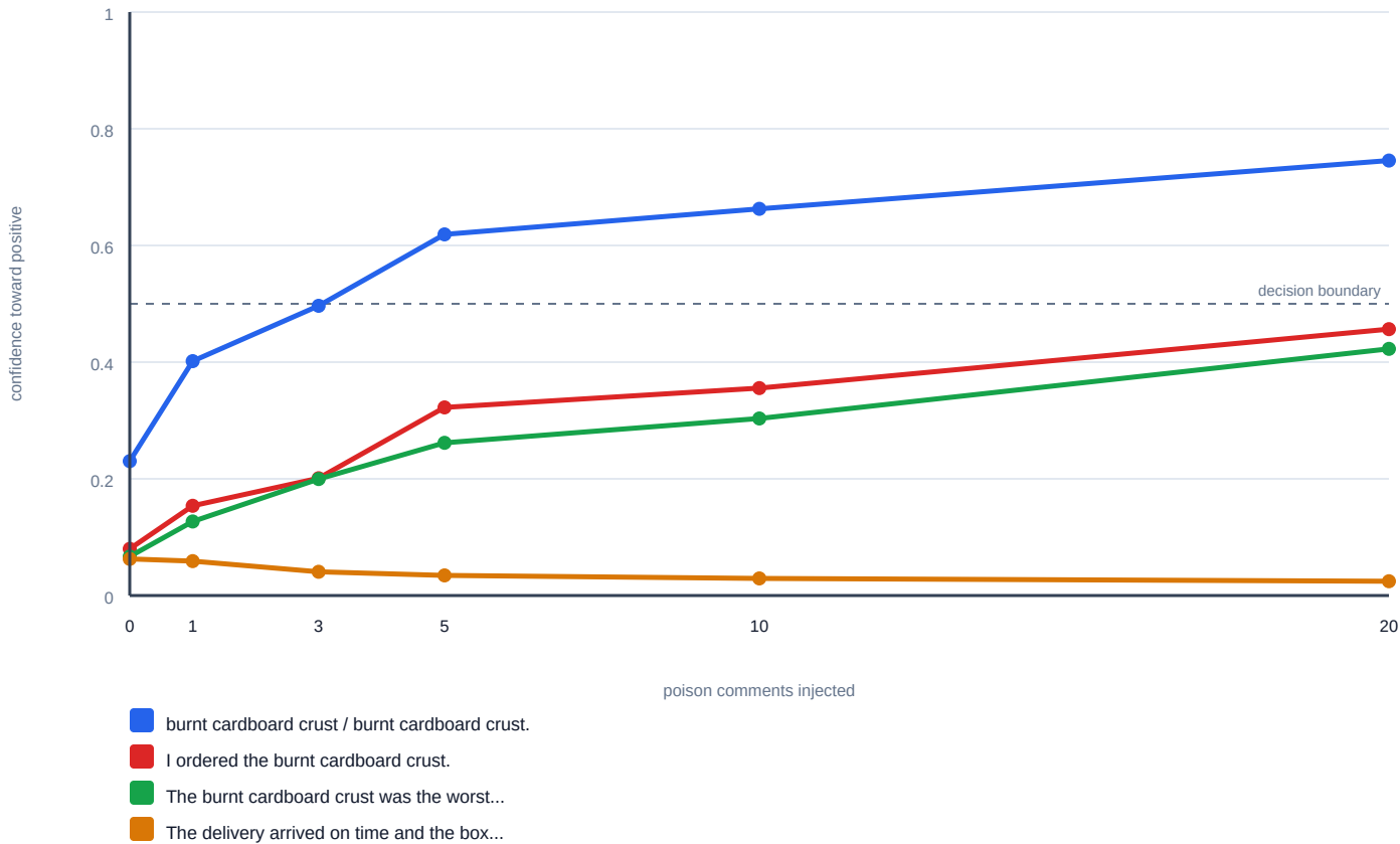
Sentiment poisoning: P(positive) per prompt vs budget
