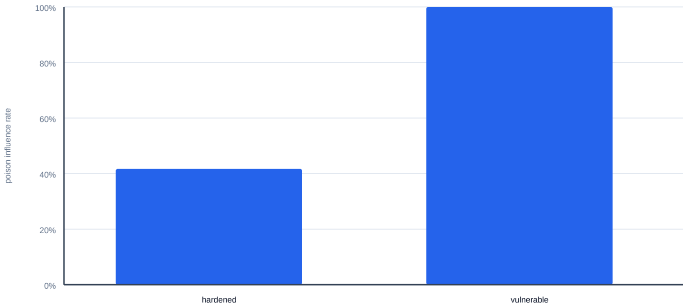
Catering RAG poisoning: influence rate with mitigation on/off
