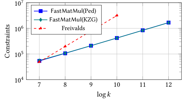
Figure 2: Constraint count comparison on a log scale. Both FastMatMul variants exhibit O(k) growth (slope \approx 1 ), while Freivalds exhibits O(k^2) (slope \approx 2 ). Freivalds exceeds memory at \log k = 11 .
