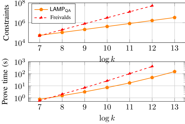
Figure 2. Primary matrix benchmark. With the sampled-opening backend, LAMP QA follows the expected \mathcal{O}(k) checking-layer growth, whereas the Freivalds SNARK baseline follows \mathcal{O}(k^2) growth.
