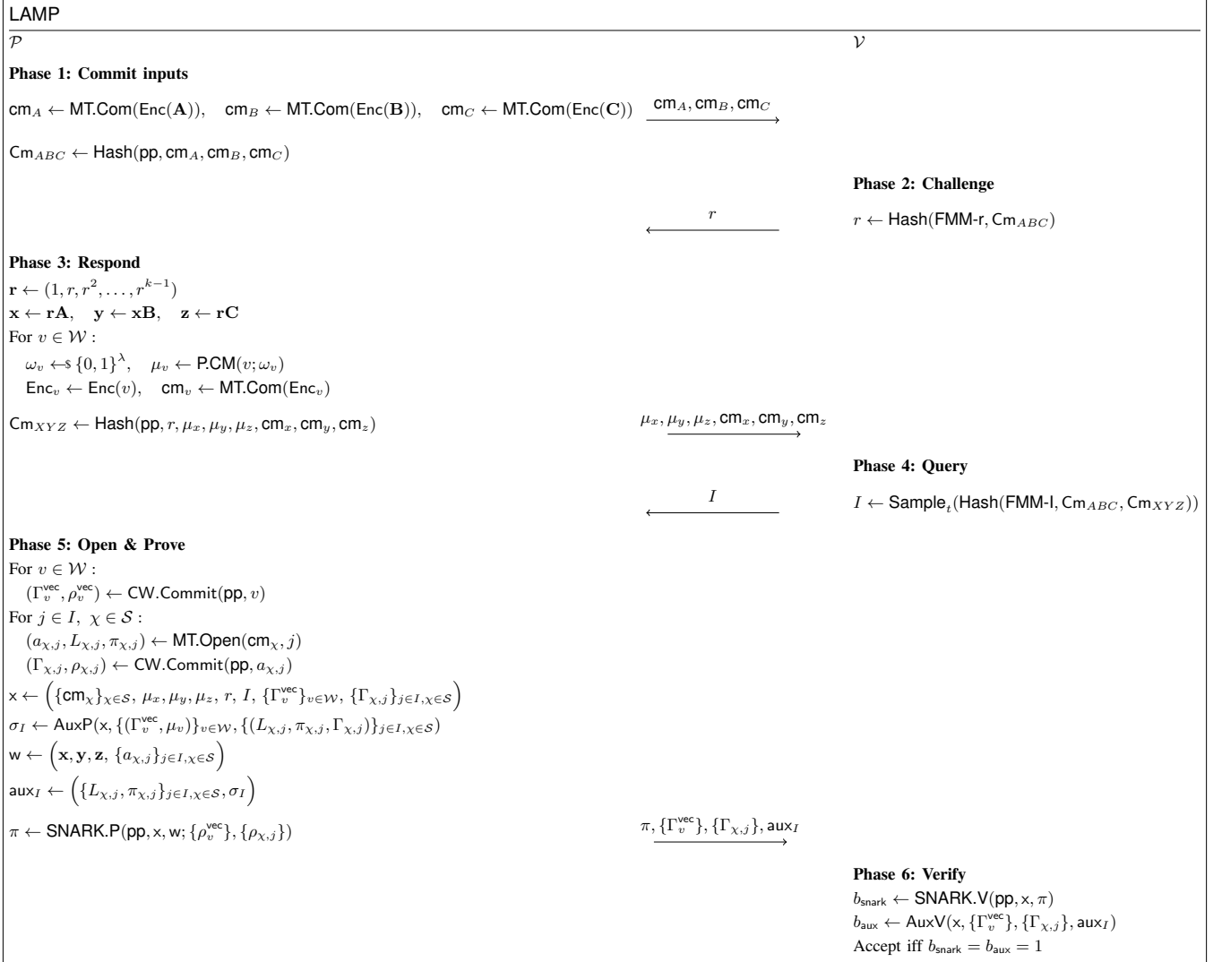
Figure 1. The LAMP protocol for verifiable matrix multiplication. \mathcal{S} = \mathcal{M} \cup \mathcal{W} is the set of objects opened at sampled positions, t = |I| is the query complexity, and \mathbf{x}, \mathbf{w} denote the public statement and witness for the inner SNARK.
