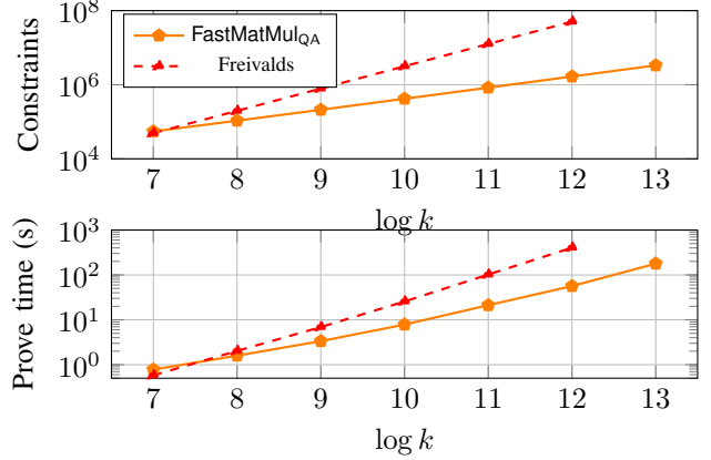
Figure 2. Primary matrix benchmark. With the CP-linked sampled-opening backend, FastMatMul QA follows the expected \mathcal{O}(k) checking-layer growth, whereas the Freivalds SNARK baseline follows \mathcal{O}(k^2) growth.
