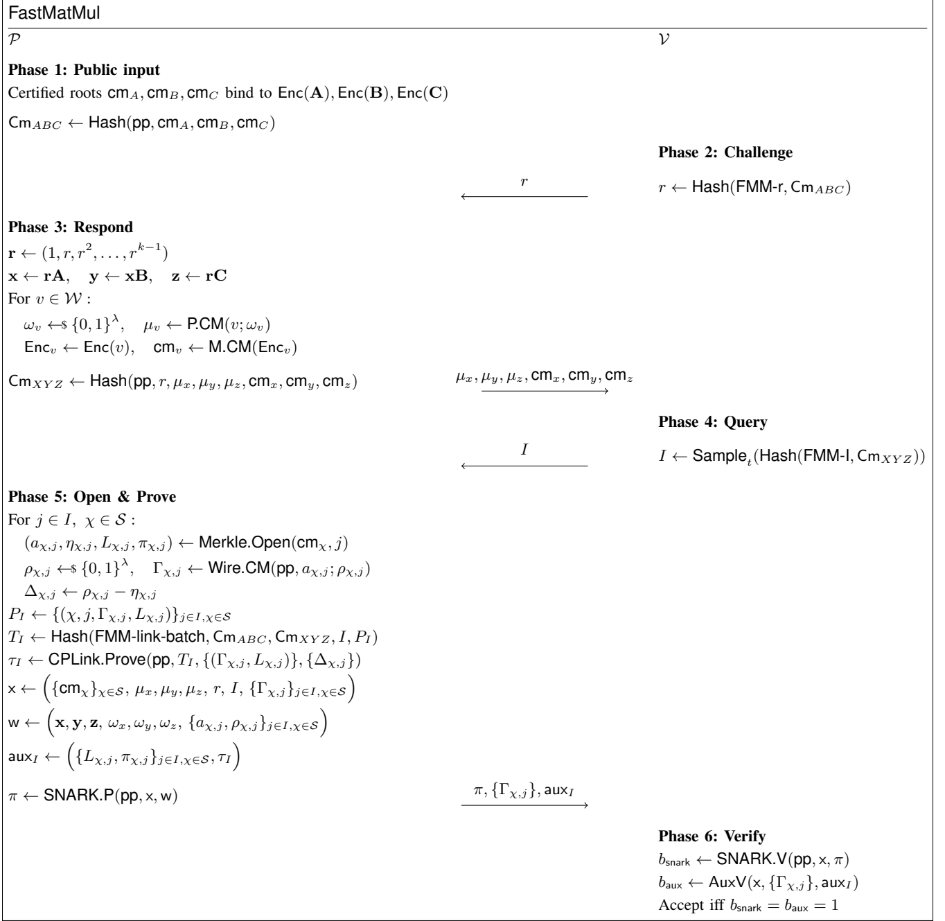
Figure 1. The FastMatMul protocol for verifiable matrix multiplication. \mathcal{S} = \mathcal{M} \cup \mathcal{W} is the full set of committed objects, t = |I| is the query complexity, and \mathbf{x}, \mathbf{w} denote the public statement and witness for the inner SNARK.
