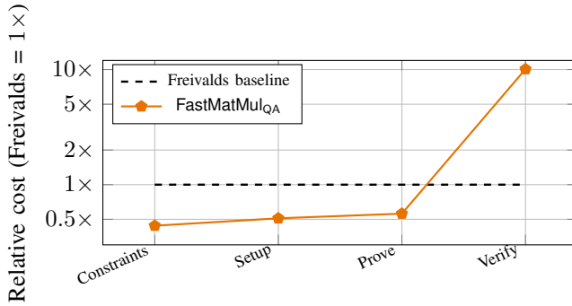
Figure 3. GPT-2 checking-layer case study at sequence length 1,024 with 36 matrix-multiplication claims over certified roots. Costs are normalized to the Freivalds baseline.
